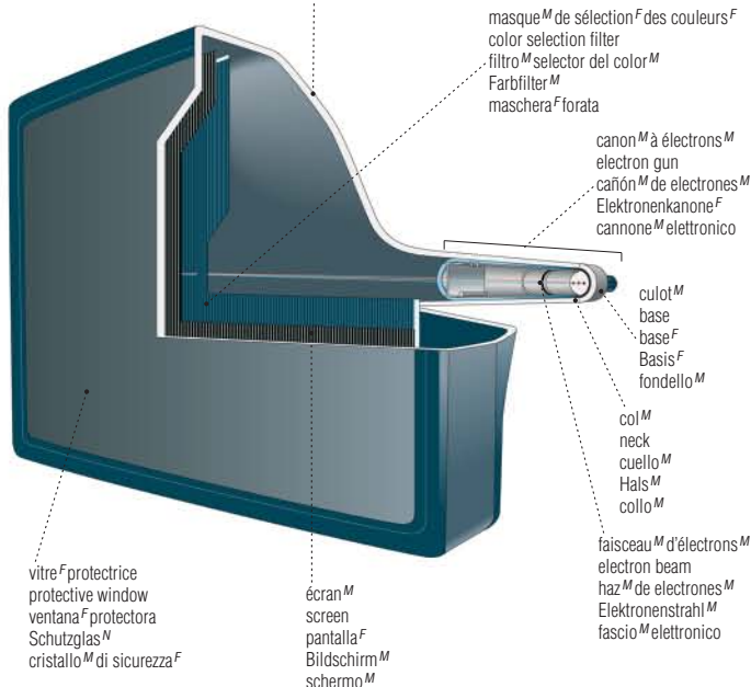
tube M -image F picture tube tubo M de pantalla F Bildröhre F cinescopio M
